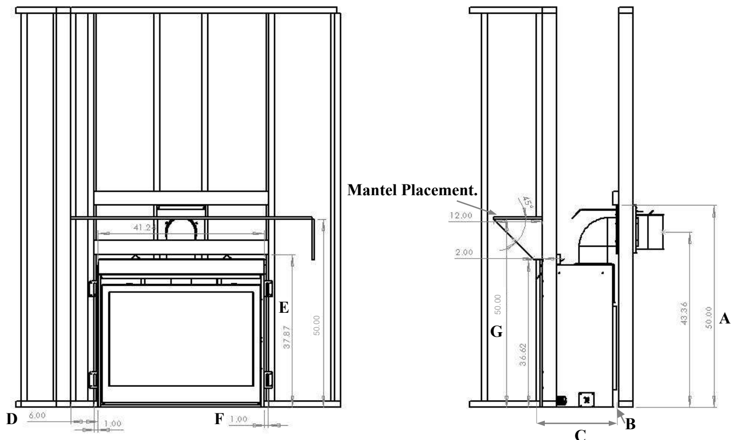
FRAMING DIMENSIONS (SEE PAGE 7) 43.34" W x 37.75" H x 19" D MINIMUM CLEARANCES TO COMBUSTIBLES TOP VENT
