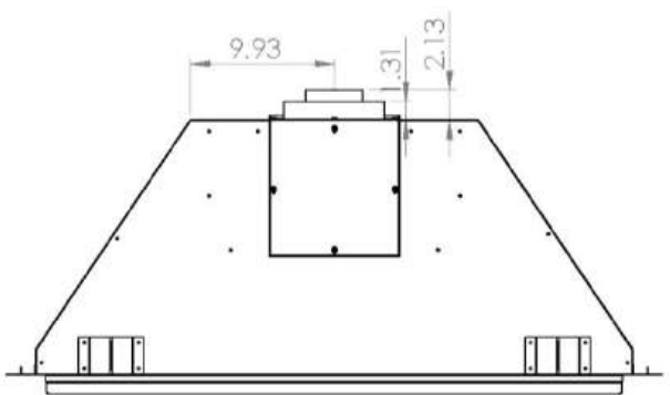
REAR VENT
